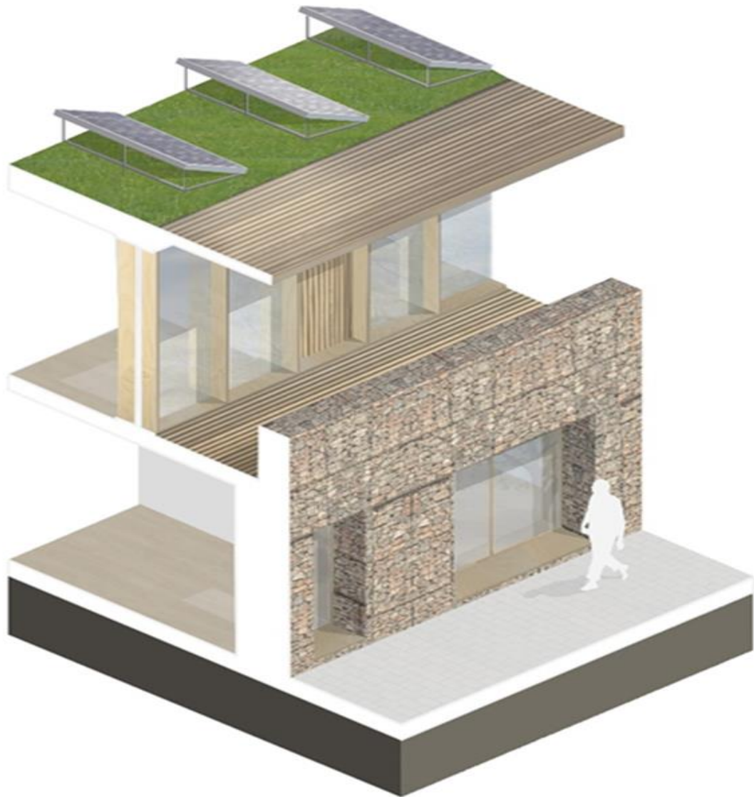
Figure 33.8 Axonometric of the gateway building facade
