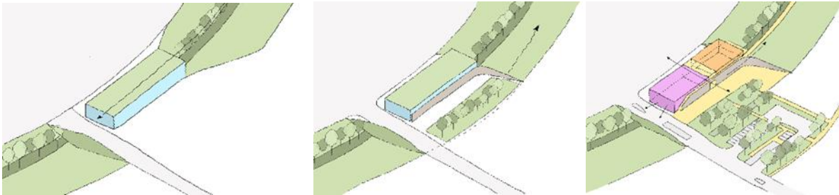
Figure 33.7 Concept sketches for the integration of the Gateway Building into the earth bank
