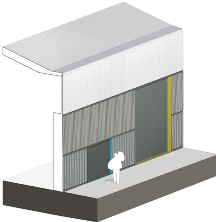
Figure 33.11 Axonometric of the Workshop Building 3-tier façade
